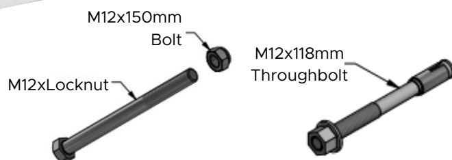
Fixings Required (Figure 1)
